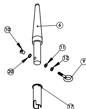
Detail "A"
