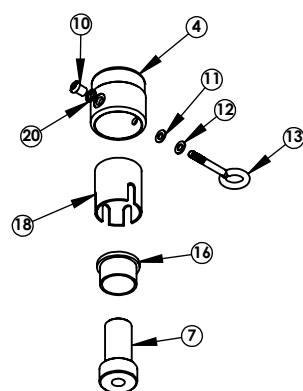
Detail "B"
